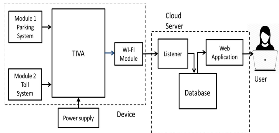
Figure 1. The Prototype Of The System.
