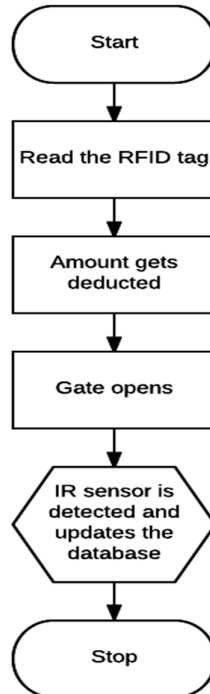
Figure 3. Exit System Of The Parking Space
